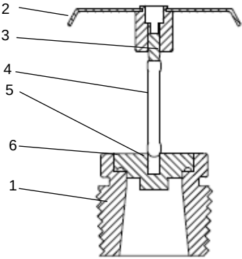
FIGURE 1 MODEL GS213, 11.2 K-FACTOR, UPRIGHT SPRINKLER STANDARD RESPONSE
