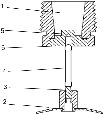
FIGURE 2 MODEL GS214, 11.2 K-FACTOR, PENDANT SPRINKLER STANDARD RESPONSE
