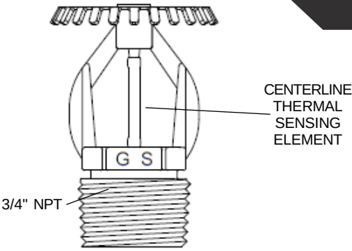
FIGURE 1 MODEL GS213, 11.2 K-FACTOR, UPRIGHT SPRINKLER STANDARD RESPONSE
