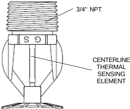
FIGURE 2 MODEL GS214, 11.2 K-FACTOR, PENDANT SPRINKLER STANDARD RESPONSE
