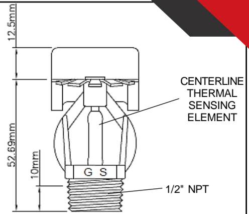
MODEL GS256, 5.6 K-FACTOR, HORIZONTAL SIDEWALL SPRINKLER STANDARD RESPONSE
