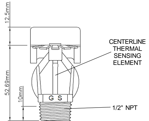
MODEL GS258, 5.6 K-FACTOR, HORIZONTAL SIDEWALL SPRINKLER QUICK RESPONSE
